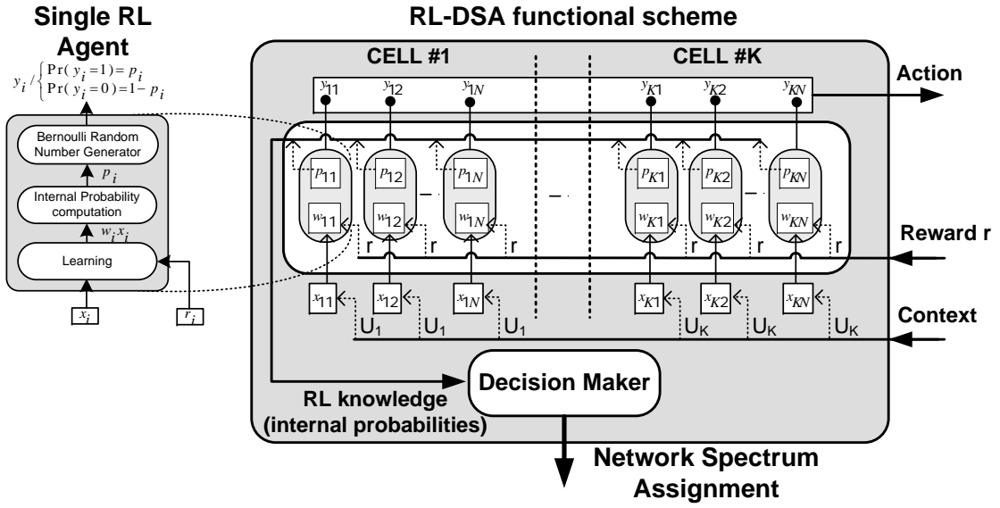
Fig. 1. RL-DSA algorithm functional scheme.
