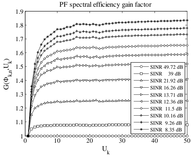
Fig. 3. Sample of considered curves for spectral efficiency gain factor of a PF scheduler over a RR scheduler.
