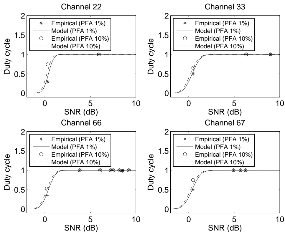
Fig. 9. Validation of duty cycle model for digital TV channels.
