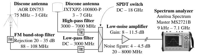
Fig. 1. Measurement setup employed in this study.
