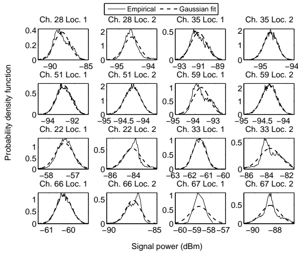
Fig. 6. Probability density function of signal power for analogical (28, 35, 51 and 59) and digital (22, 33, 66 and 67) TV channels.
