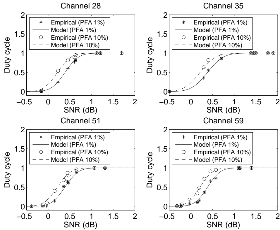
Fig. 8. Validation of duty cycle model for analogical TV channels.
