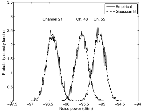
Fig. 5. Probability density function of noise power measured at different TV channels.
