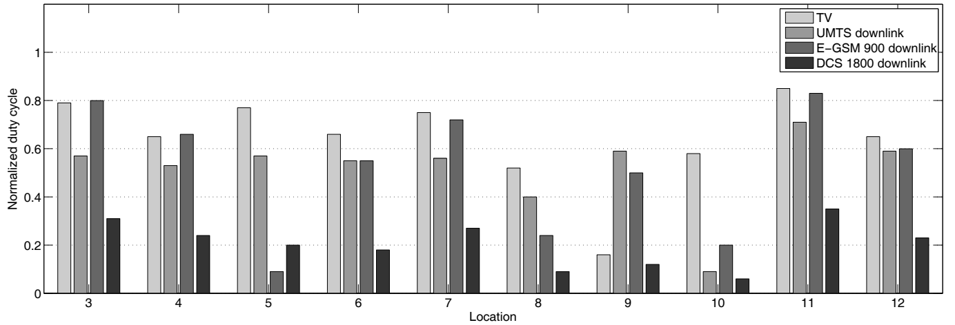
Fig. 4. Normalized average duty cycle statistics in locations 3 to 12 for specific bands: TV (470-862 MHz), UMTS downlink (2110-2170 MHz), E-GSM 900 downlink (925-960 MHz), and DCS 1800 downlink (1805-1880 MHz).
