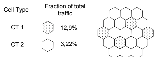
Fig. 3: Simulation model.
