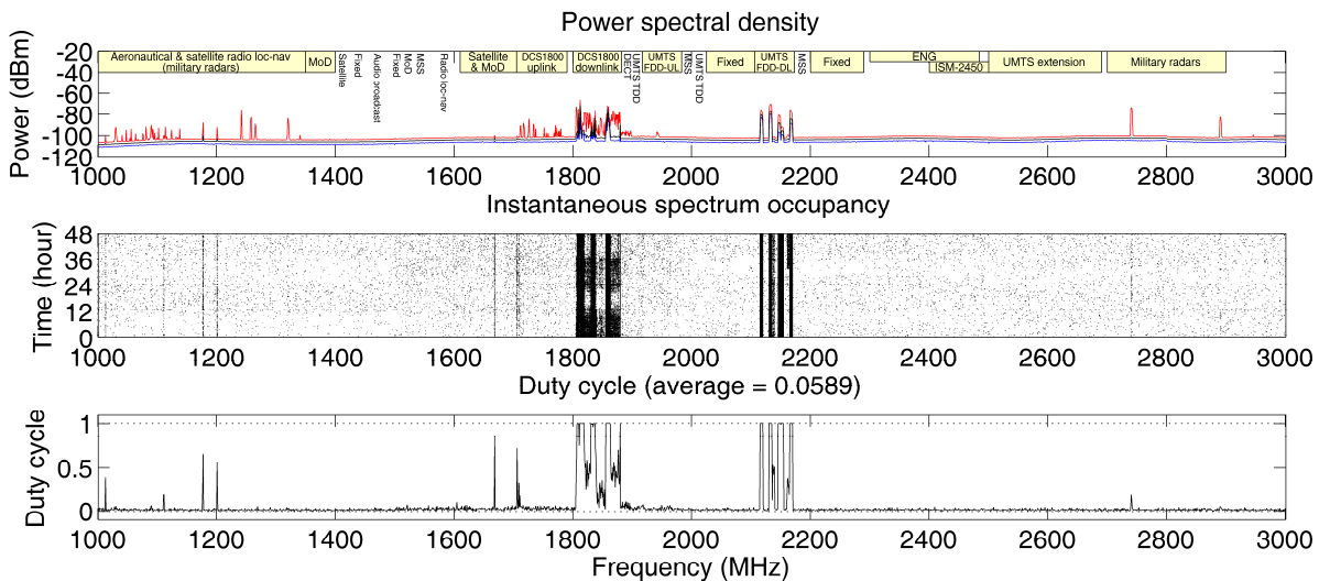
Figure 2. Occupancy results between 1000 and 3000 MHz.
