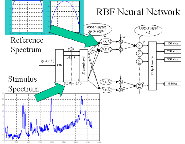
Figure 4. The radial basis functional neural network (RBF NN).
