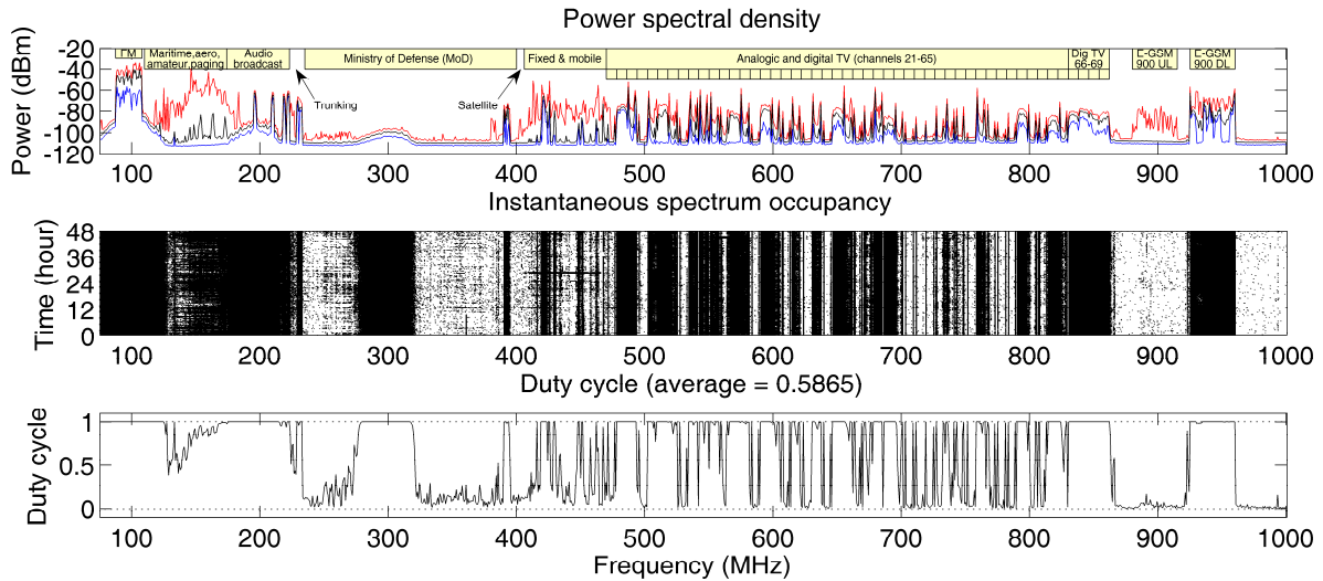
Figure 1. Occupancy results between 75 and 1000 MHz.
