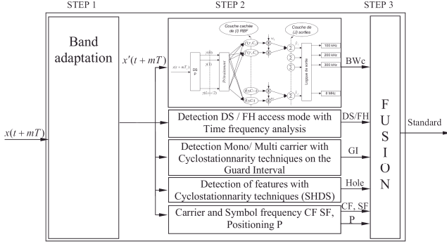
Figure 3. The new standard recognition sensor.
