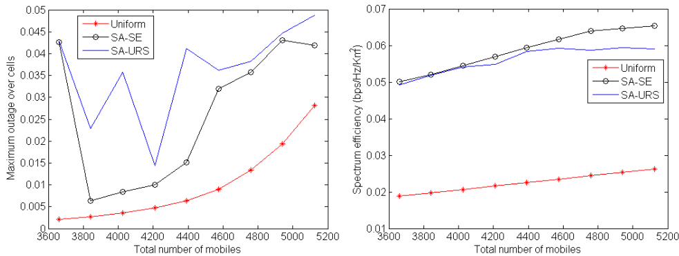
Figure 4: Outage probability (left) and spectrum efficiency (right) as a function of the total number of users
