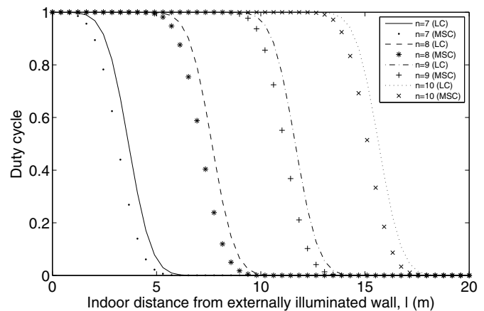
Fig. 9. Perceived spectrum occupancy at indoor locations ( P_T = 60 dBm, \sigma_S = 0.5252 dB, \sigma_N = 0.1679 dB, P_{fa} = 0.01 , NF = 8.6 dB, d = 5 km, b = 40 m, w = 20 m, h_b = 50 m, h_r = 40 m, h_m = 2 m).
