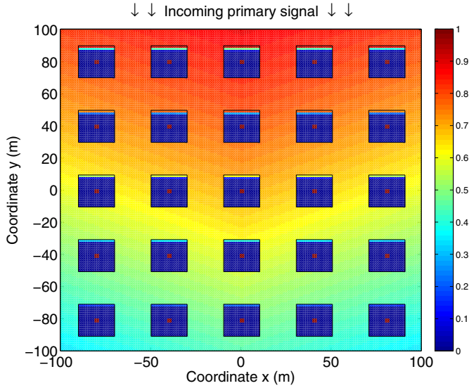
Fig. 5. Probabilistic spectrum occupancy pattern perceived at various locations within the area under study ( P_T = 60 dBm, \sigma_S = 0.5252 dB, \sigma_N = 0.1679 dB, P_{fa} = 0.01 , NF = 8.6 dB, d = 4.8 km, b = 40 m, w = 20 m, h_b = 50 m, h_r = 40 m, h_m = 2 m, n = 3 ).
