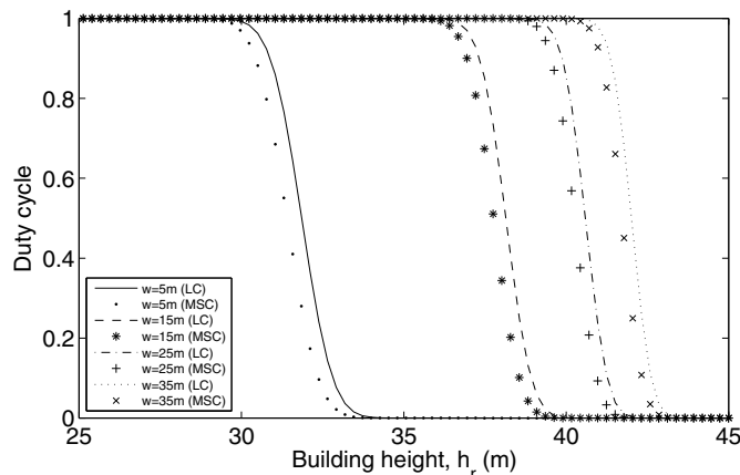
Fig. 8. Perceived spectrum occupancy at the ground level ( P_T = 60 dBm, \sigma_S = 0.5252 dB, \sigma_N = 0.1679 dB, P_{fa} = 0.01 , NF = 8.6 dB, d = 5 km, h_b = 50 m, h_m = 2 m).
