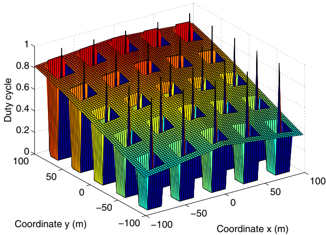
Fig. 6. Probabilistic spectrum occupancy pattern perceived at various locations within the area under study ( P_T = 60 dBm, \sigma_S = 0.5252 dB, \sigma_N = 0.1679 dB, P_{fa} = 0.01 , NF = 8.6 dB, d = 4.8 km, b = 40 m, w = 20 m, h_b = 50 m, h_r = 40 m, h_m = 2 m, n = 3 ).
