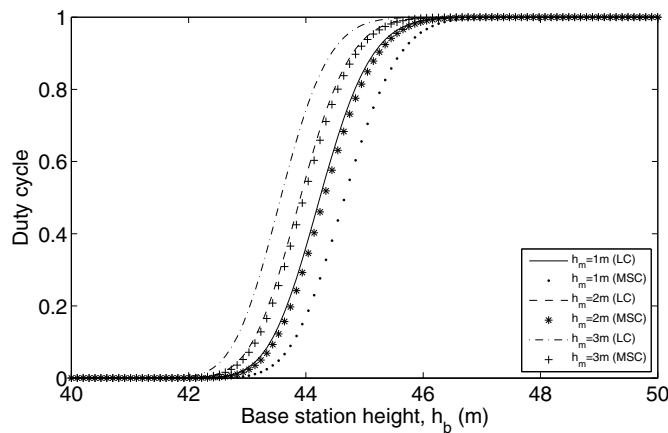
Fig. 7. Perceived spectrum occupancy at the ground level ( P_T = 60 dBm, \sigma_S = 0.5252 dB, \sigma_N = 0.1679 dB, P_{fa} = 0.01 , NF = 8.6 dB, d = 5 km, b = 40 m, w = 20 m, h_r = 35 m).
