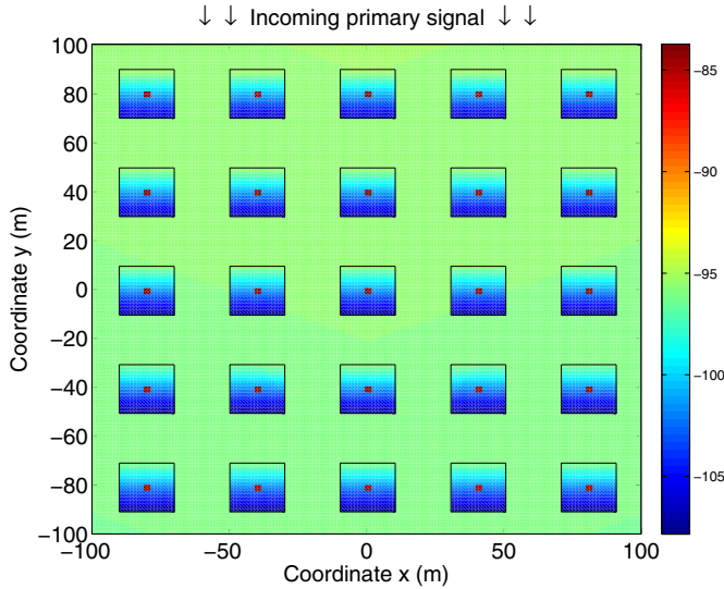
Fig. 3. Primary signal power P_S (dBm) received at various locations within the area under study ( P_T = 60 dBm, \sigma_S = 0.5252 dB, \sigma_N = 0.1679 dB, d = 4.8 km, b = 40 m, w = 20 m, h_b = 50 m, h_r = 40 m, h_m = 2 m, n = 3 ).
