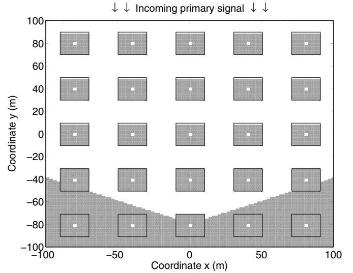
Fig. 4. Binary spectrum occupancy pattern perceived at various locations within the area under study ( P_T = 60 dBm, \sigma_S = 0.5252 dB, \sigma_N = 0.1679 dB, P_{fa} = 0.01 , NF = 8.6 dB, d = 4.8 km, b = 40 m, w = 20 m, h_b = 50 m, h_r = 40 m, h_m = 2 m, n = 3 ).
