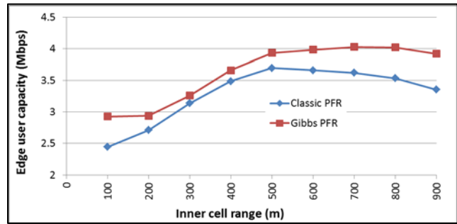
Figure 5: Average Edge User Capacity
