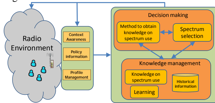
Figure 1: General framework for spectrum selection
